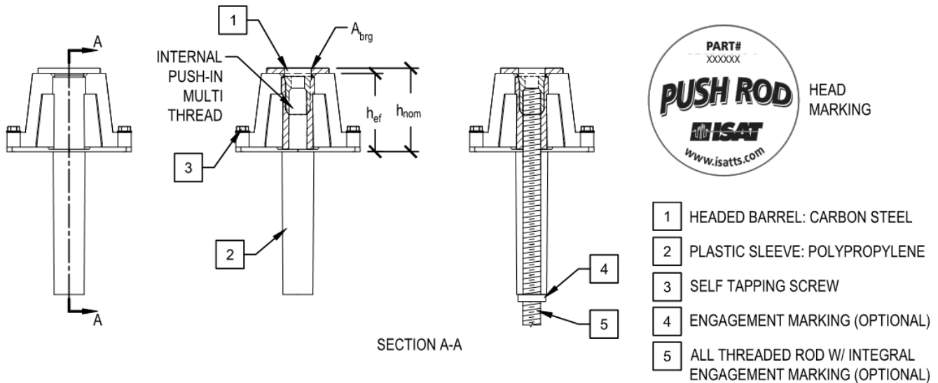
FIGURE 2B—PR-SDI3812-2 CAST-IN-PLACE INSERTS FOR CONCRETE OVER METAL DECKS
