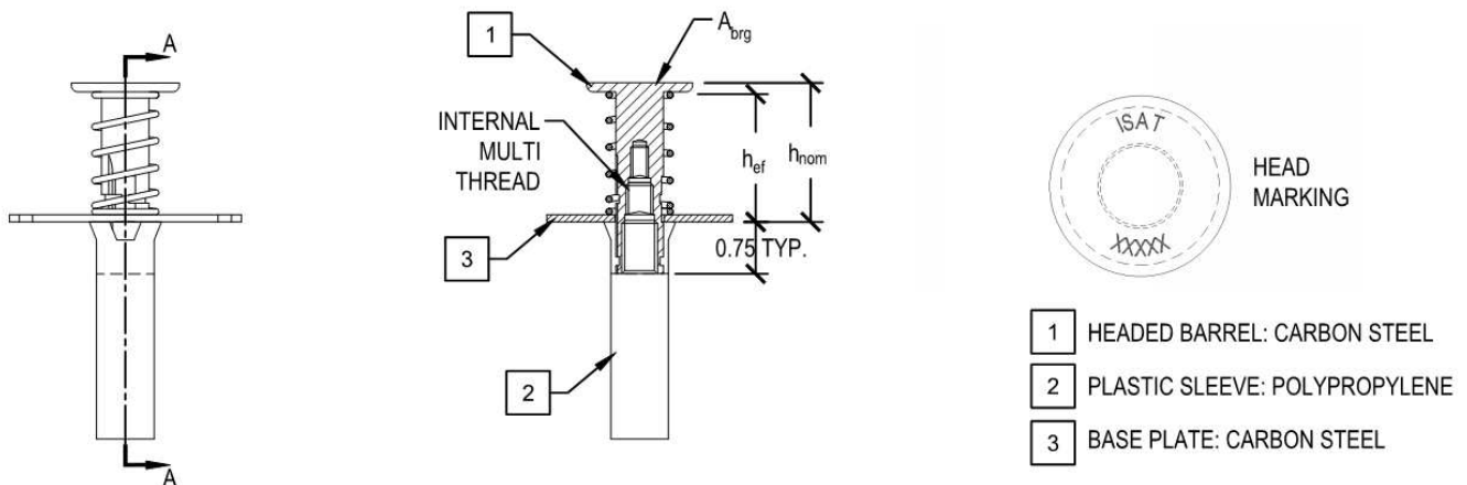
FIGURE 3A—SDI CAST-IN-PLACE INSERTS FOR CONCRETE OVER METAL DECKS
