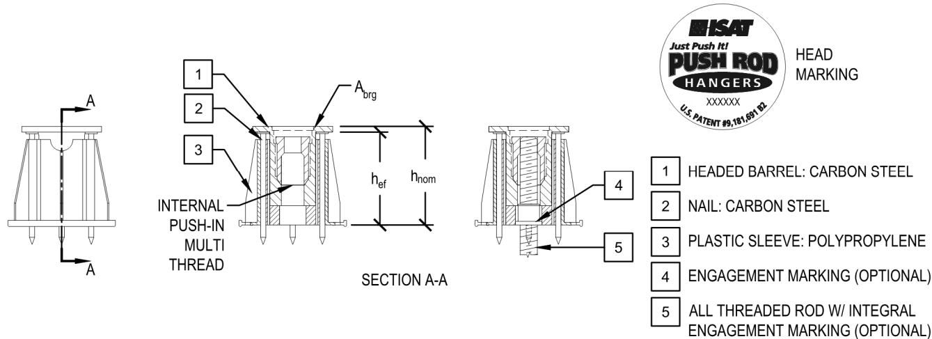
FIGURE 1B—ISAT-PRPIP3812 CAST-IN-PLACE INSERTS FOR FORM POUR CONCRETE
